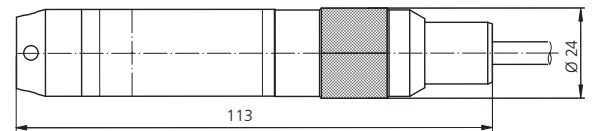
Fig. 4 open, screwable version
